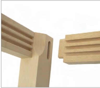
Mortise and Tenon Joints
