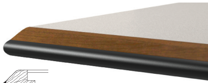
38177 1.25" x 1.25" beveled wood edge 1/2" vinyl T mold edge, black high pressure laminate, veneer, or Veneer Art top surface
