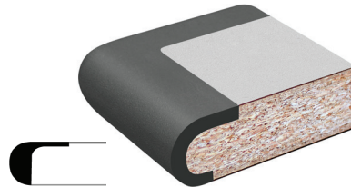
71111 1.25" x 1.75" molded urethane fused edge full bullnose edge high pressure laminate top surface several colors available, see finishes
